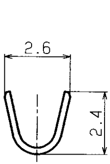
WIRE BARREL
